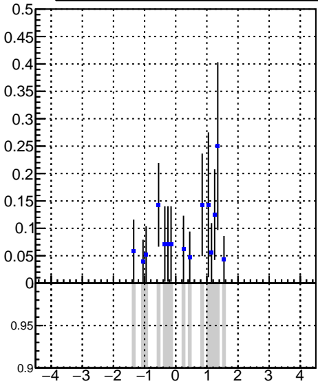
DQM_V0001_R000000001_Global_CMSSW_X.Y.Z_RECO
