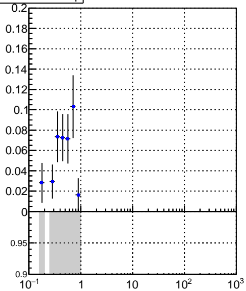
DQM_V0001_R000000001_Global_CMSSW_X_Y_Z_RECO
