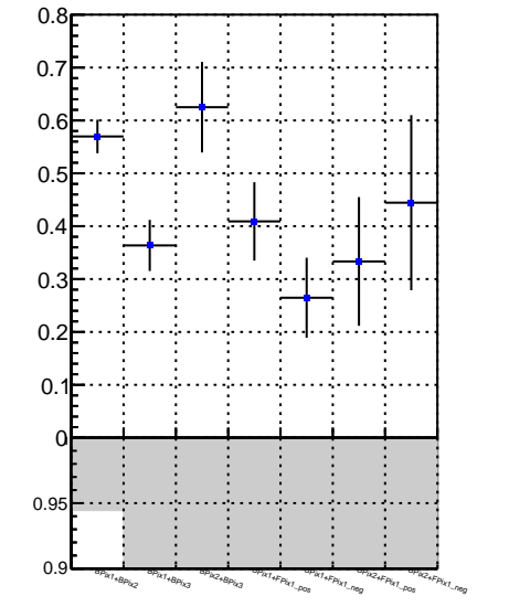
Fake rate vs. DQM_V0001_R000000001_Global_CMSSW_X_Y_Z_RECO
