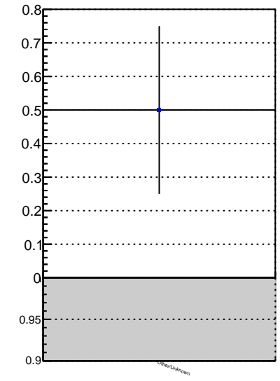
Fake rate vs. —●— DQM_V0001_R00000001_Global_CMSSW_X_Y_Z_RECO
