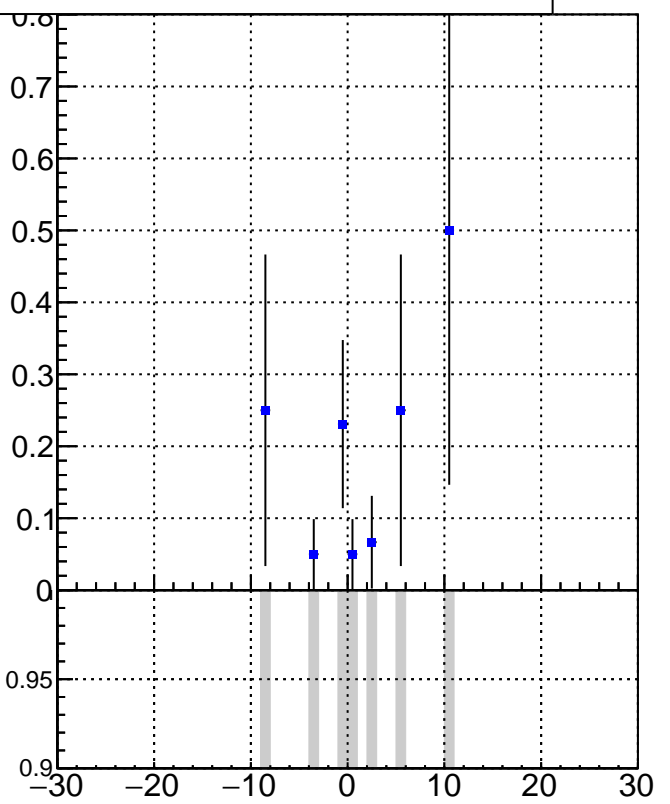
DQM_V0001_R000000001_Global_CMSSW_X_Y_Z_RECO
