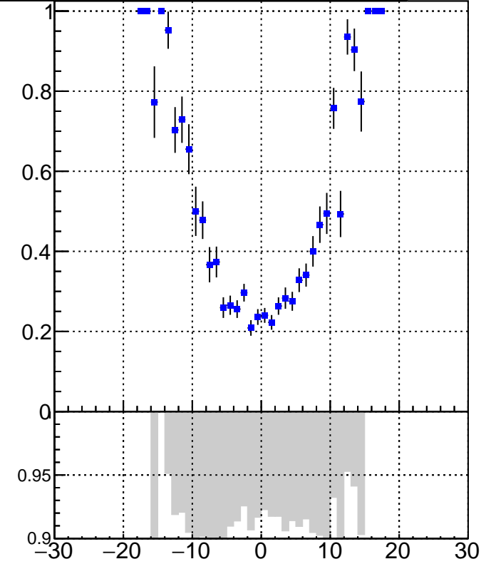
DQM_V0001_R000000001_Global_CMSSW_X_Y_Z_RECO
