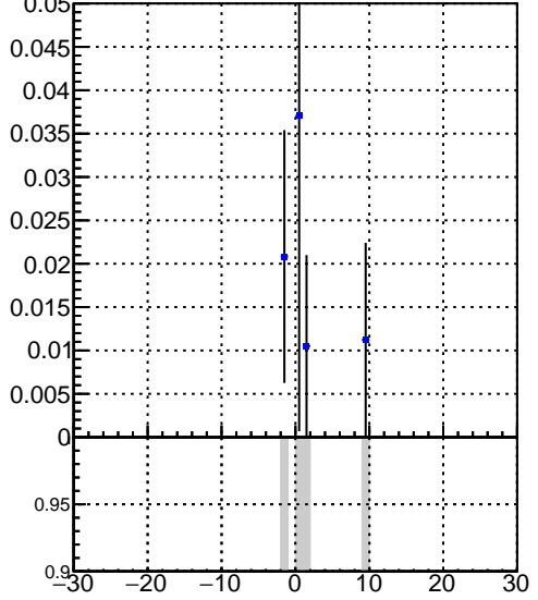
Efficiency vs sim PV z ■ DQM_V0001_R000000001_Global_CMSSW_X.Y.Z_RECO
