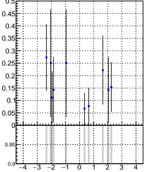
DQM_V0001_R000000001_Global_CMSSW_X.Y.Z_RECO
