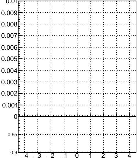
DQM_V0001_R000000001_Global_CMSSW_X.Y.Z_RECO
