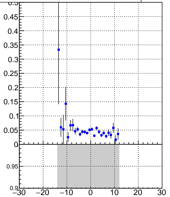
DQM_V0001_R000000001_Global_CMSSW_X_Y_Z_RECO
