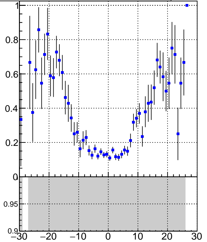
DQM_V0001_R000000001_Global_CMSSW_X_Y_Z_RECO
