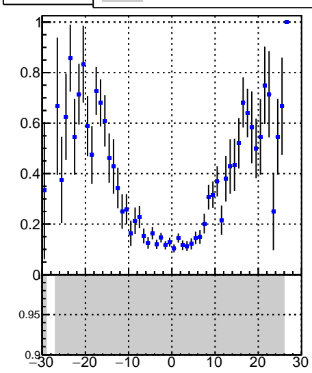
Fake rate vs \nu DQM_V0001_R000000001_Global_CMSSW_X_Y_Z_RECO
