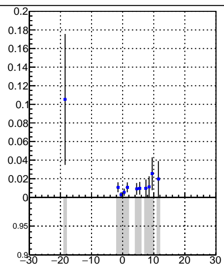
Fake rate vs \nu DQM_V0001_R000000001_Global_CMSSW_X_Y_Z_RECO
