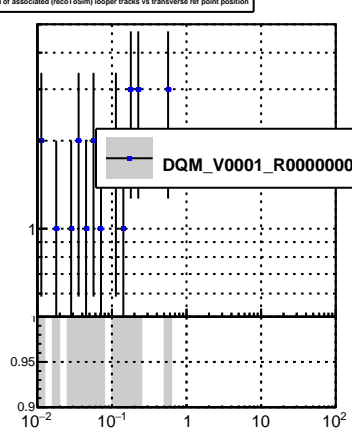
N of associated (recoToSim) looper tracks vs transverse ref point position
