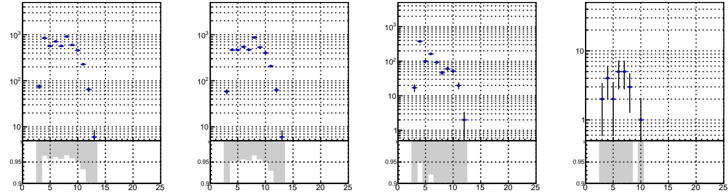
DQM_V0001_R000000001_Global_CMSSW_X_Y_Z_RECO
