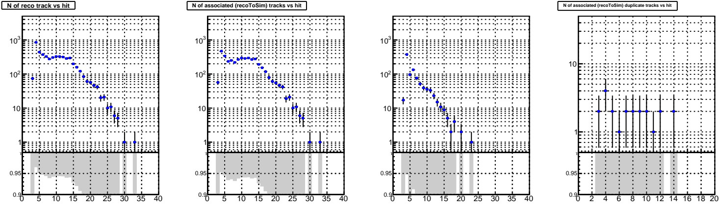
DQM_V0001_R000000001_Global_CMSSW_X_Y_Z_RECO
