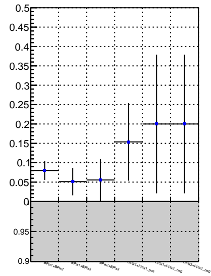
Fake rate vs. DQM_V0001_R000000001_Global_CMSSW_X_Y_Z_RECO
