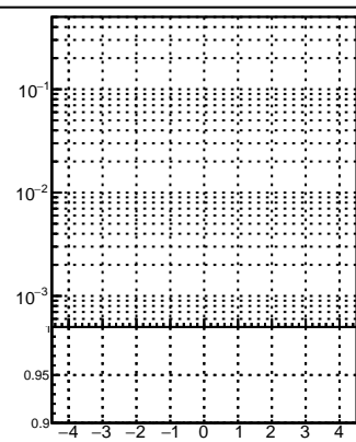
DQM_V0001_R00000001_Global_CMSSW_X_Y_Z_RECO
