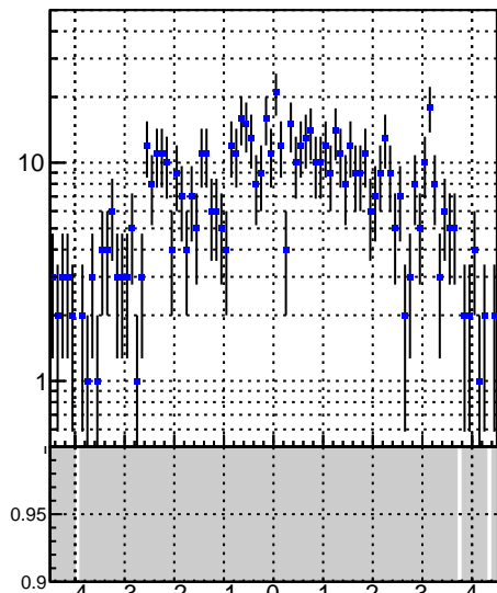
N of simulated tracks vs phi
