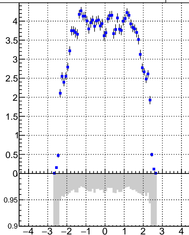
DQM_V0001_R000000001_Global_CMSSW_X_Y_Z_RECO
