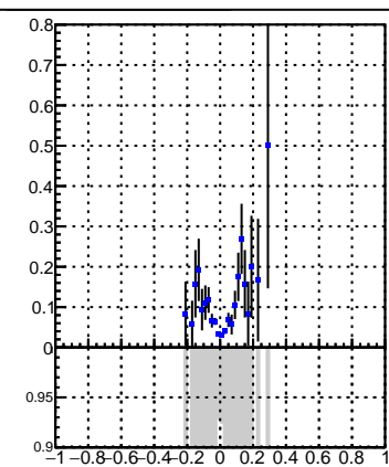
DQM_V0001_R000000001_Global_CMSSW_X_Y_Z_RECO
