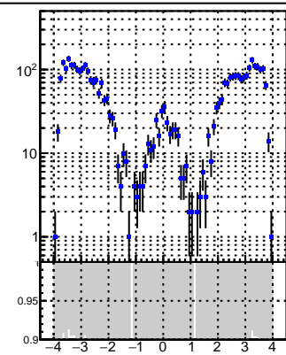
DQM_V0001_R000000001_Global_CMSSW_X_Y_Z_RECO
