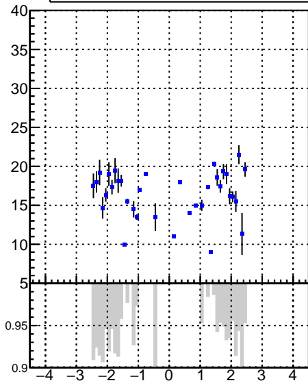
mean hit DQM_V0001_R000000001_Global_CMSSW_X.Y.Z_RECO
