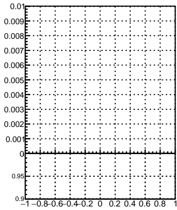
DQM_V0001_R000000001_Global_CMSSW_X_Y_Z_RECO
