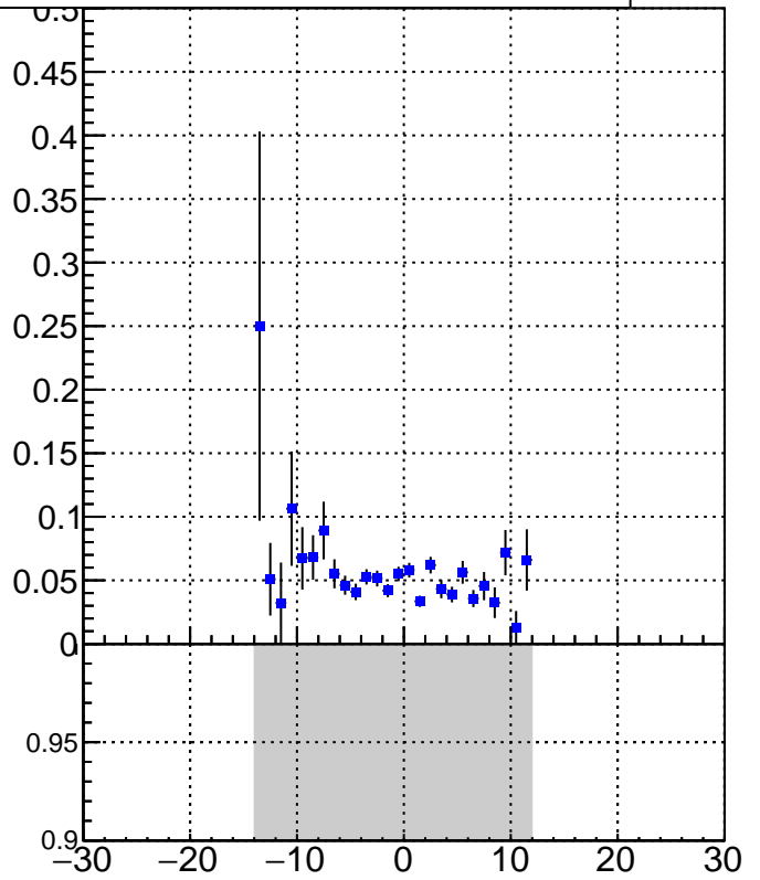
DQM_V0001_R000000001_Global_CMSSW_X_Y_Z_RECO
