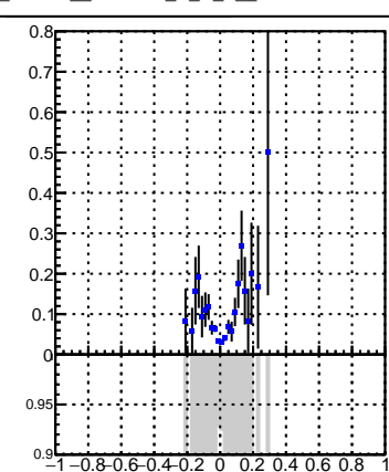
DQM_V0001_R000000001_Global_CMSSW_X_Y_Z_RECO
