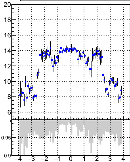
mean hit DQM_V0001_R000000001_Global_CMSSW_X_Y_Z_RECO
