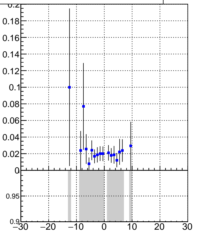
DQM_V0001_R000000001_Global_CMSSW_X_Y_Z_RECO
