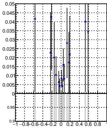
DQM_V0001_R000000001_Global_CMSSW_X_Y_Z_RECO
