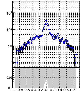
DQM_V0001_R000000001_Global_CMSSW_X_Y_Z_RECO
