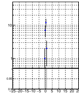
DQM_V0001_R000000001_Global_CMSSW_X_Y_Z_RECO
