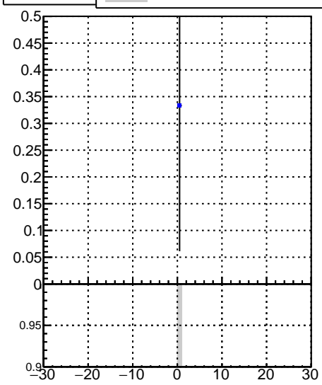
Fake rate vs v_z DQM_V0001_R000000001_Global_CMSSW_X_Y_Z_RECO
