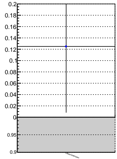
Fake rate vs. DQM_V0001_R000000001_Global_CMSSW_X_Y_Z_RECO
