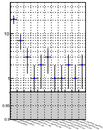
N of reco track vs. \chi^2 DQM_V0001_R000000001_Global_CMSSW_X_Y_Z_RECO
