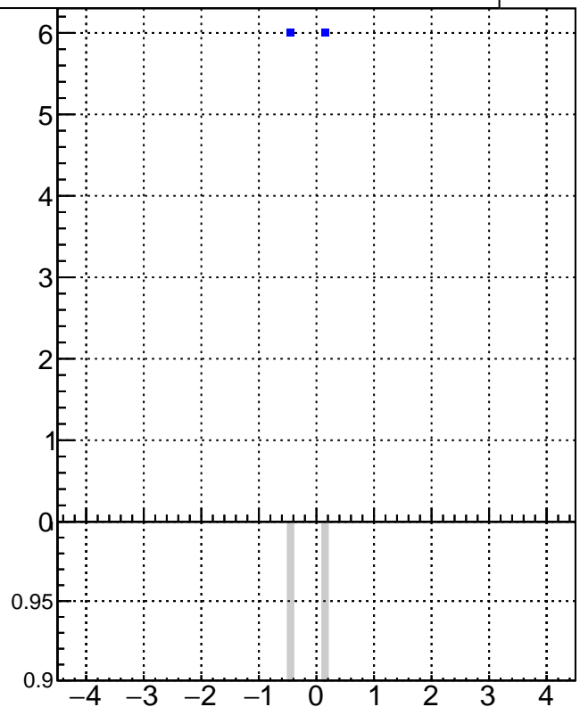
DQM_V0001_R000000001_Global_CMSSW_X_Y_Z_RECO
