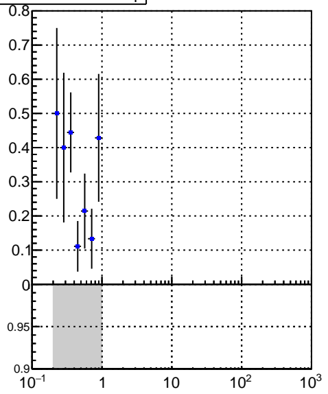
DQM_V0001_R000000001_Global_CMSSW_X_Y_Z_RECO
