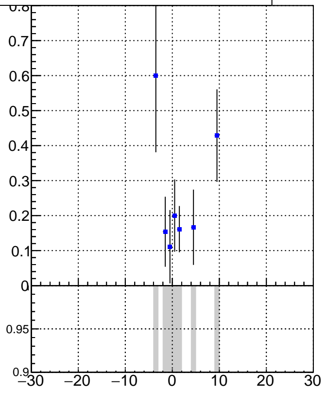
DQM_V0001_R000000001_Global_CMSSW_X_Y_Z_RECO
