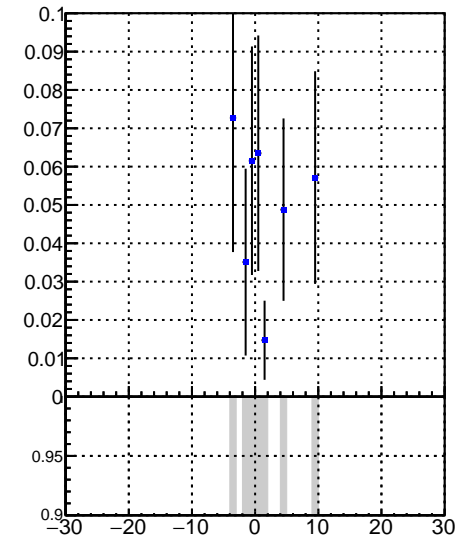
Fake rate vs dxy DQM_V0001_R000000001_Global_CMSSW_X_Y_Z_RECO
