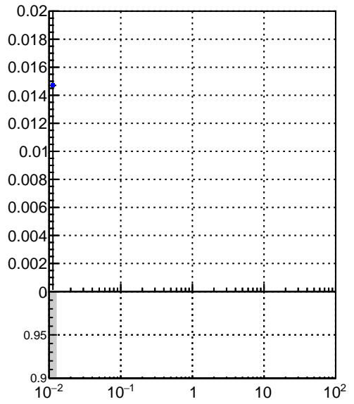
DQM_V0001_R000000001_Global_CMSSW_X_Y_Z_RECO
