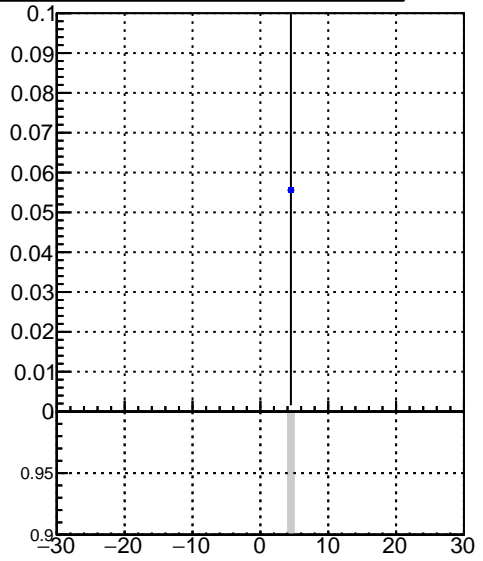
DQM_V0001_R000000001_Global_CMSSW_X_Y_Z_RECO
