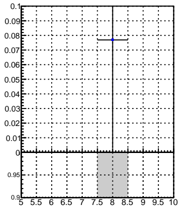
DQM_V0001_R000000001_Global_CMSSW_X_Y_Z_RECO
