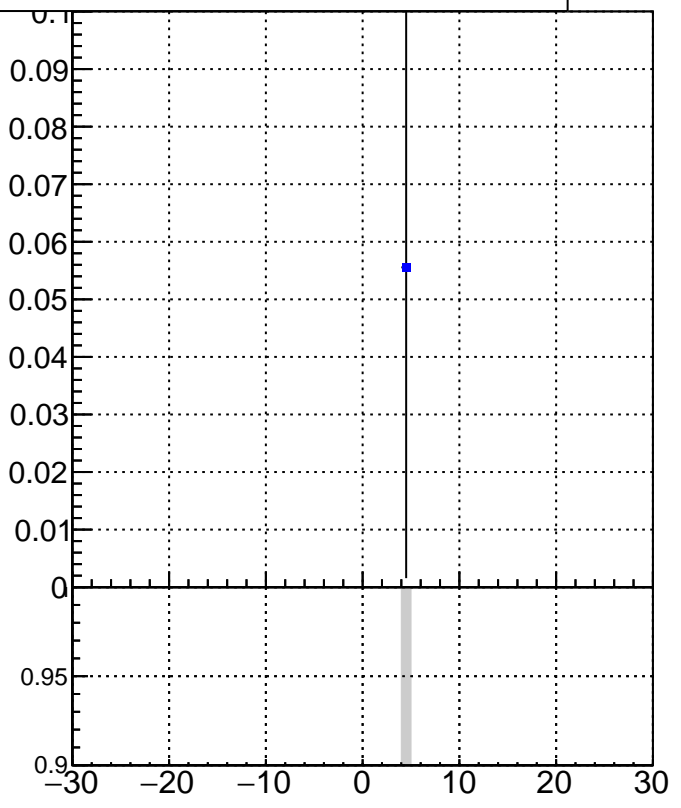
DQM_V0001_R000000001_Global_CMSSW_X_Y_Z_RECO
