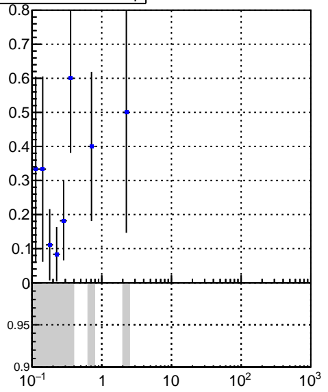
DQM_V0001_R000000001_Global_CMSSW_X_Y_Z_RECO
