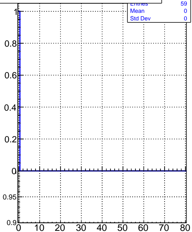
DQM_V0001_R000000001_Global_CMSSW_X_Y_Z_RECO
