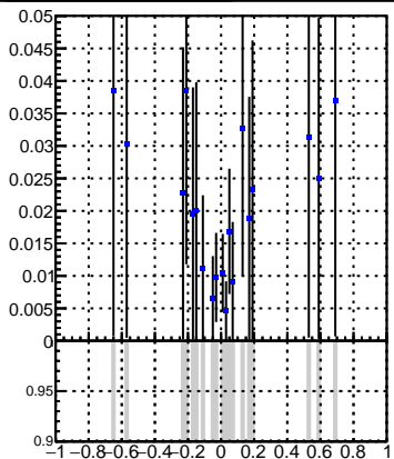
DQM_V0001_R000000001_Global_CMSSW_X_Y_Z_RECO
