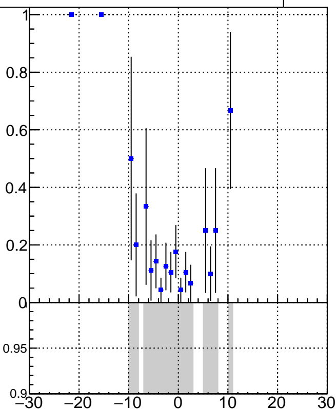
DQM_V0001_R000000001_Global_CMSSW_X_Y_Z_RECO
