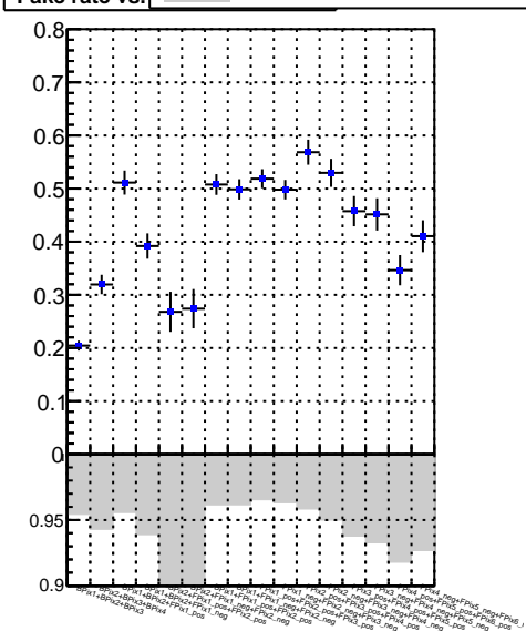
Fake rate vs. DQM_V0001_R00000001_Global_CMSSW_X_Y_Z_RECO
