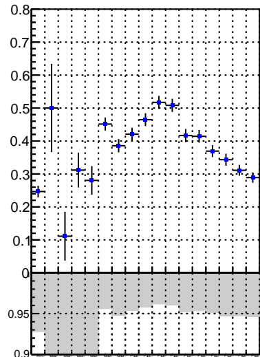
Fake rate vs. DQM_V0001_R000000001_Global_CMSSW_X_Y_Z_RECO
