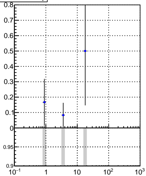
DQM_V0001_R000000001_Global_CMSSW_X.Y.Z_RECO
