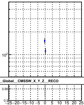
N of associated (recoToSim) tracks vs dx
