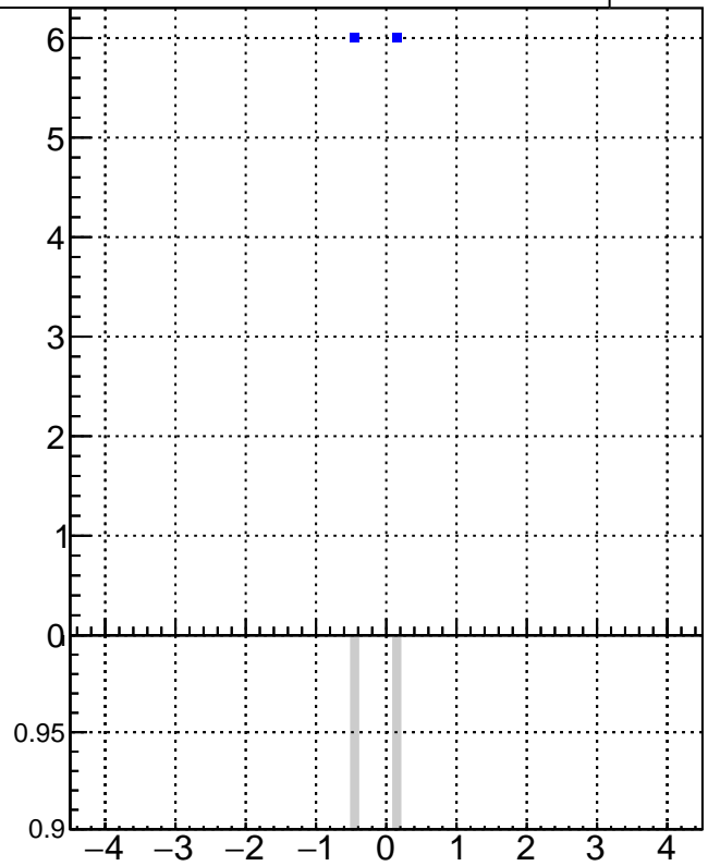
DQM_V0001_R000000001_Global_CMSSW_X_Y_Z_RECO
