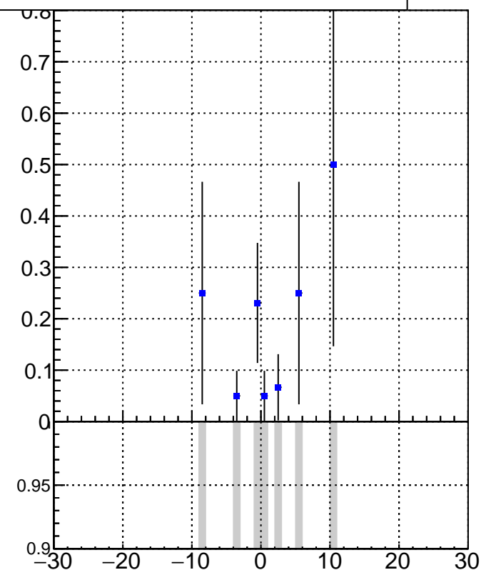
DQM_V0001_R000000001_Global_CMSSW_X_Y_Z_RECO
