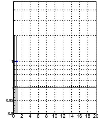
N of associated (recoToSim) looper tracks vs normalized \chi^2 DQM_V0001_R000000001_Global_CMSSW_X_Y_Z_RECO
