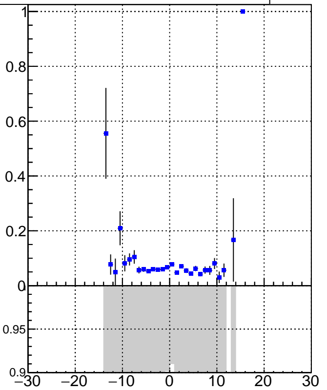
DQM_V0001_R000000001_Global_CMSSW_X_Y_Z_RECO
