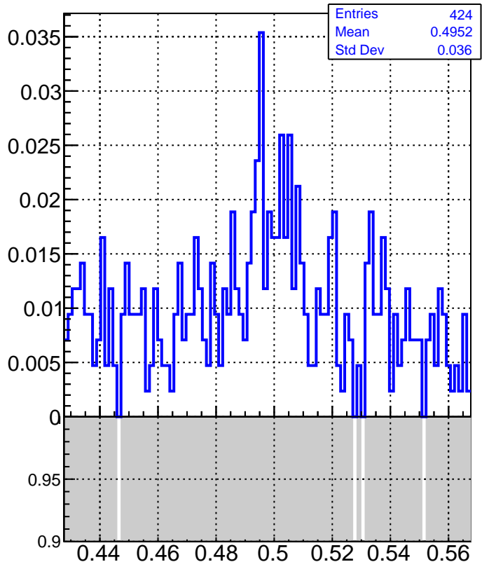
Invariant mass of all K0S
